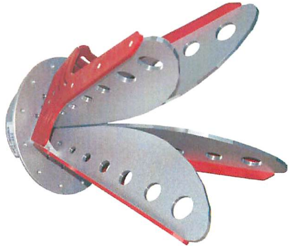
ETS-Lindgren's Model 3164-08 Quad-Ridged Horn
