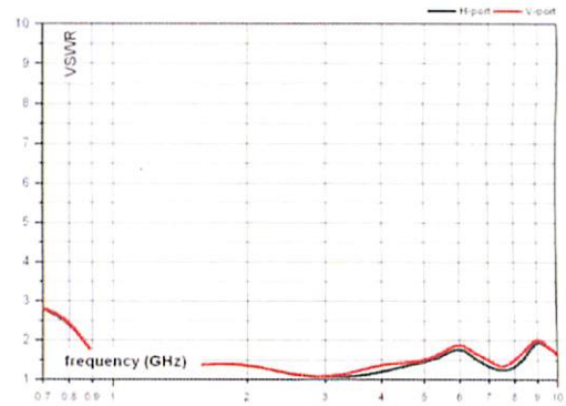
Model 3164-08 Typical VSWR
