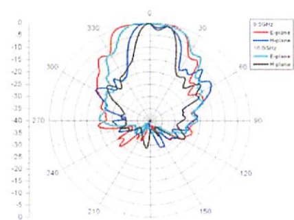
Model 3164-08 Typical 9.5 GHz to 10 GHz
