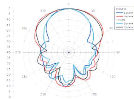
Model 3164-08 Typical 900 MHz to 1.0 GHz
