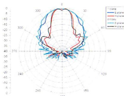
Model 3164-08 Typical 7.5 GHz to 8.0 GHz
