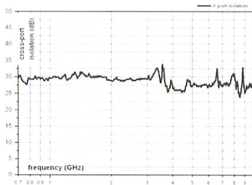
Model 3164-08 Typical Cross Port Isolation
