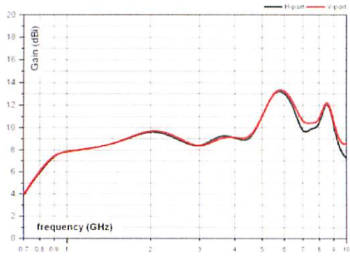
Model 3164-08 Typical Antenna Gain
