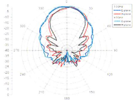
Model 3164-08 Typical 3.5 GHz to 4.0 GHz
