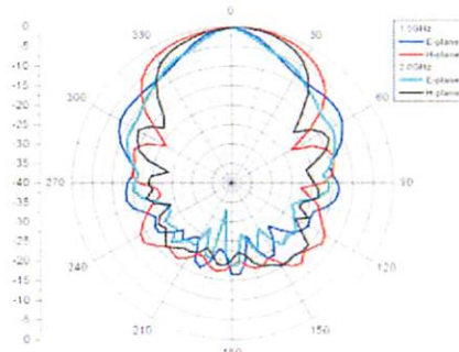
Model 3164-08 Typical 1.5 GHz to 2.0 GHz
